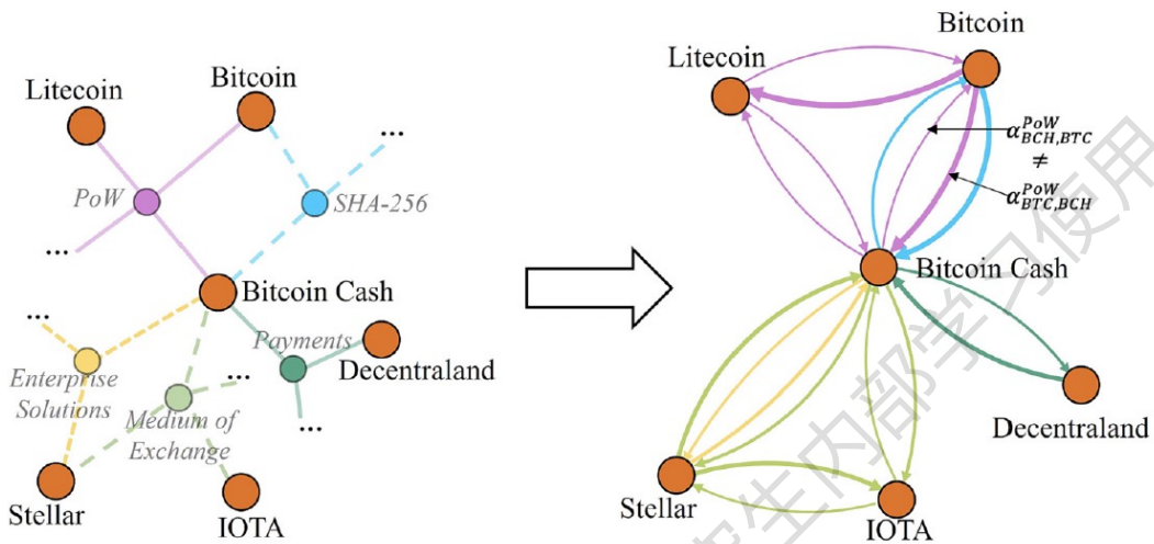
Fig. 2. An example cryptocurrency network.
